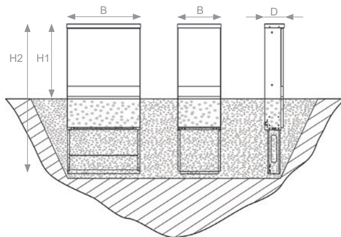
Nedgravning (Illustration)
