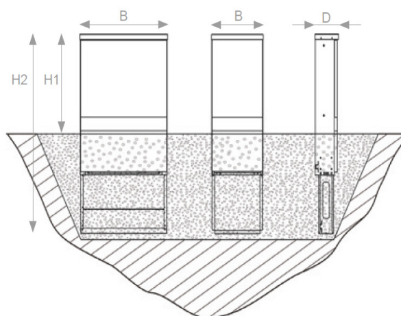
Nedgravning (Illustration)
